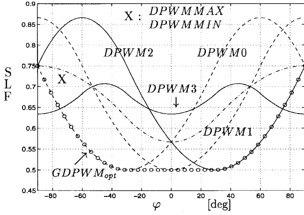
Fig. 17. SLF = f(\varphi) characteristics of the popular DPWM methods under fixed carrier frequency constraint ( SLF_{CPWM} = 1 ).
