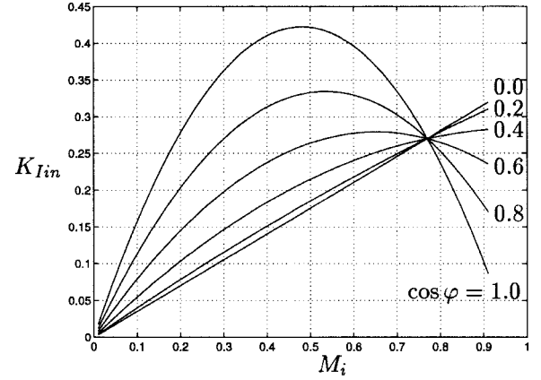
Fig. 14. Normalized inverter input harmonic current rms value characteristics K_{In} = f(M_i) of PWM-VSI for \cos \varphi as parameter.
