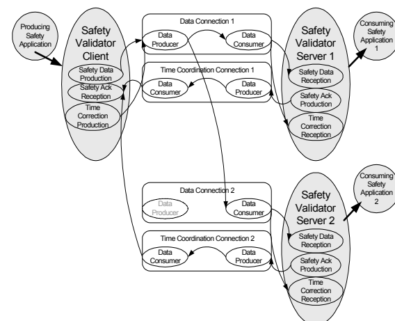
Figure 7: Multi-Cast Connection
