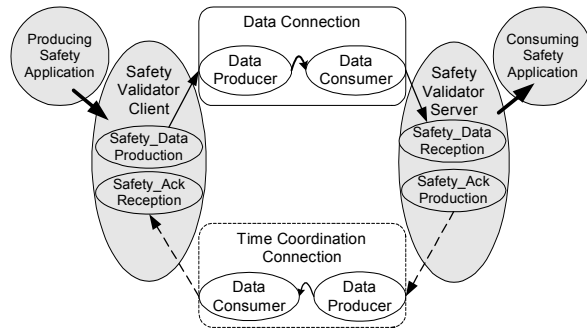
Figure 6: Single-Cast Connection
