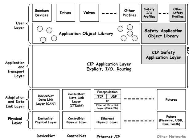
Figure 1: CIP communications layers
