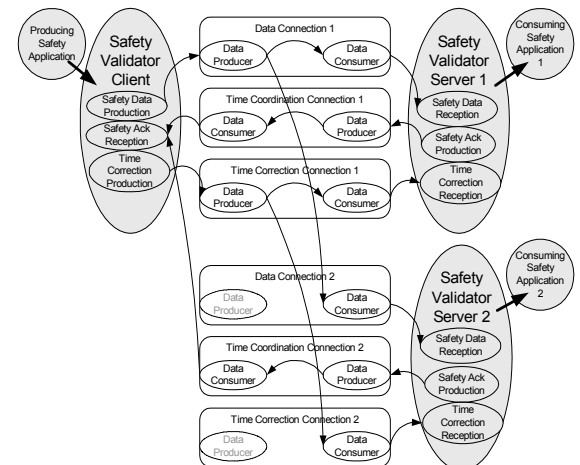
Figure 8: Multicast Connection on DeviceNet
