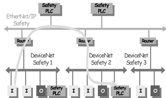
Figure 3: Network Routing
