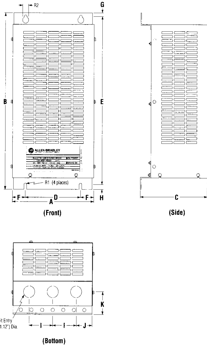
Dimensions and Weights in Millimeters (Inches) and Kilograms (Pounds)
