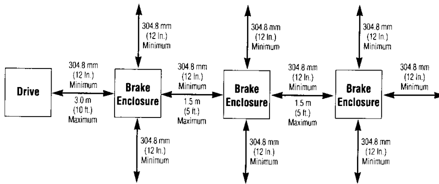
KA005-KA010, KB005-KB010 and KC005-KC010 Multiple Brake Enclosures — Recommended Maximum (3) —
