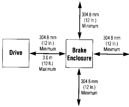
Single Brake Enclosure
