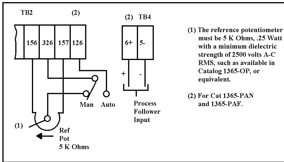
Figure 1.4 Reference Signal Connection
