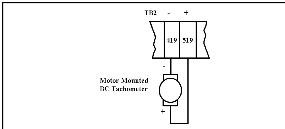
Figure 1.5 DC Tachometer Connection
