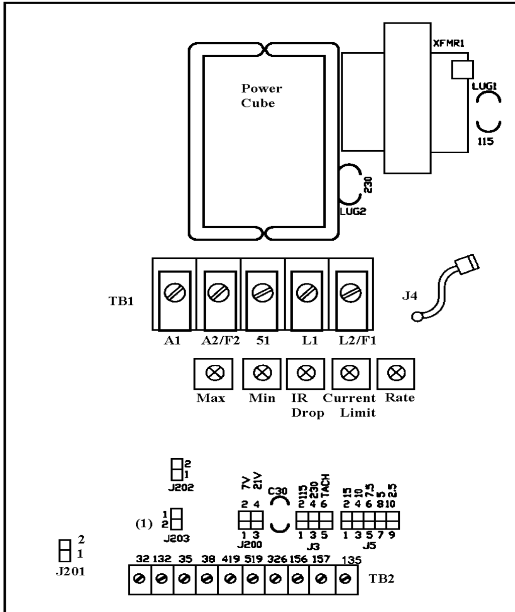
Figure 1.6 Controller Terminal Board Locations ( Catalog 1365-SAN, 1365-SAF, and 1365-DAF).
