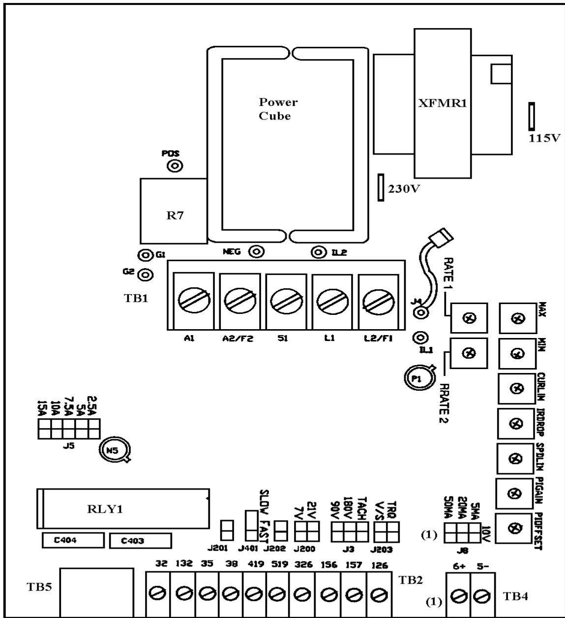
Figure 1.7 Controller Terminal Board Locations for Catalog 1365-TAN, 1365-PAF, and 1365-TAF.
