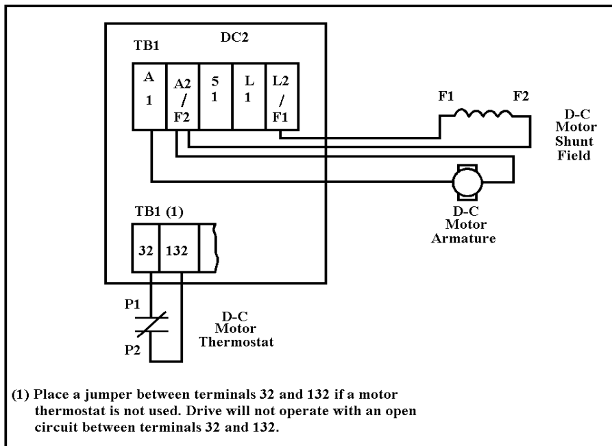
Figure 1.1 Armature, Field and Thermostat ( CCW Rotation ) Connections.
