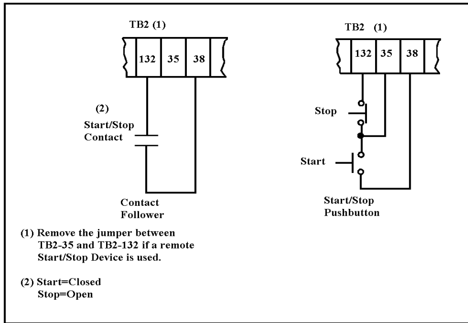
Figure 1.2 Start/Stop Circuit Connection.
