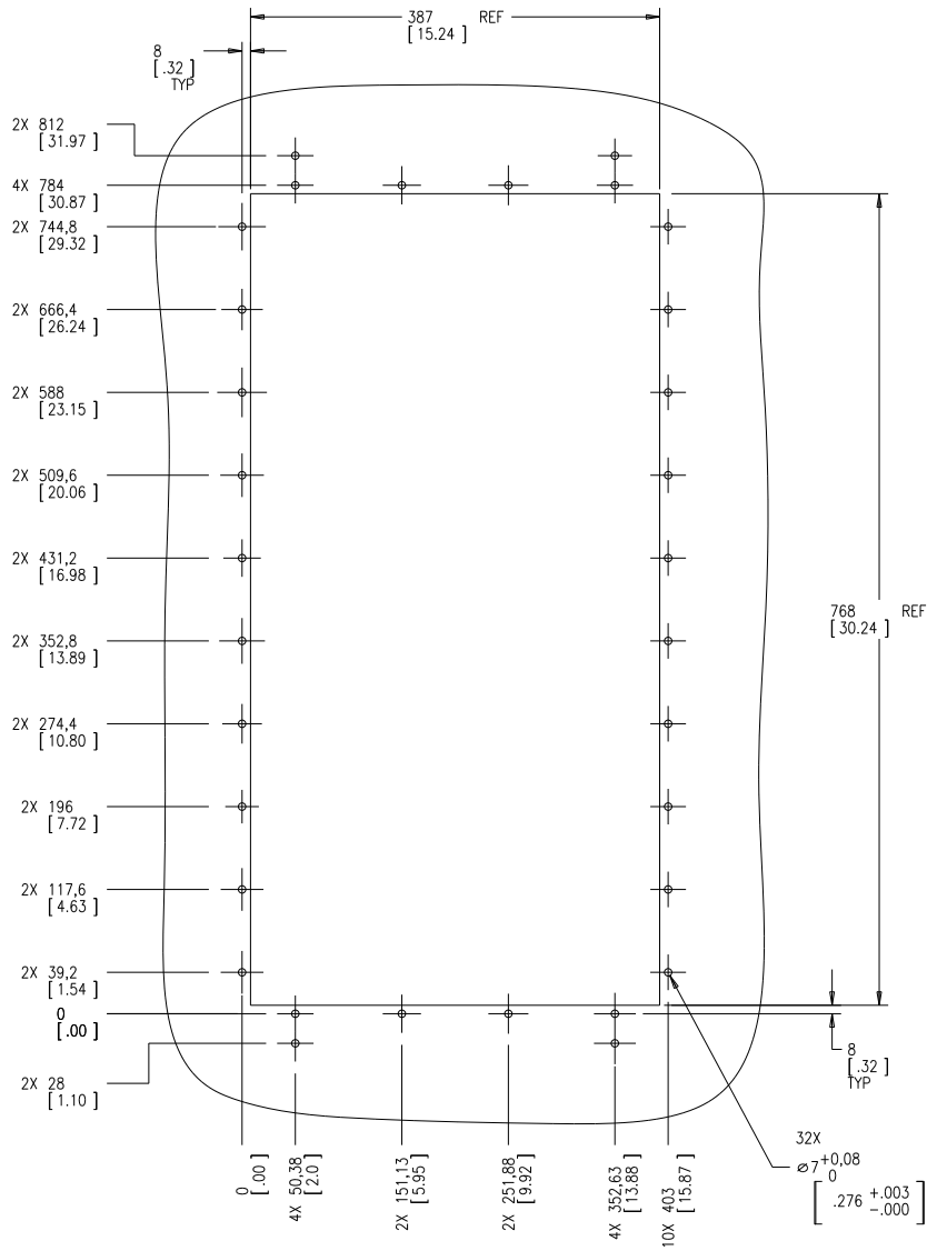
FLANGE MOUNT DRIVE PANEL CUTOUT SCALE 0.375
