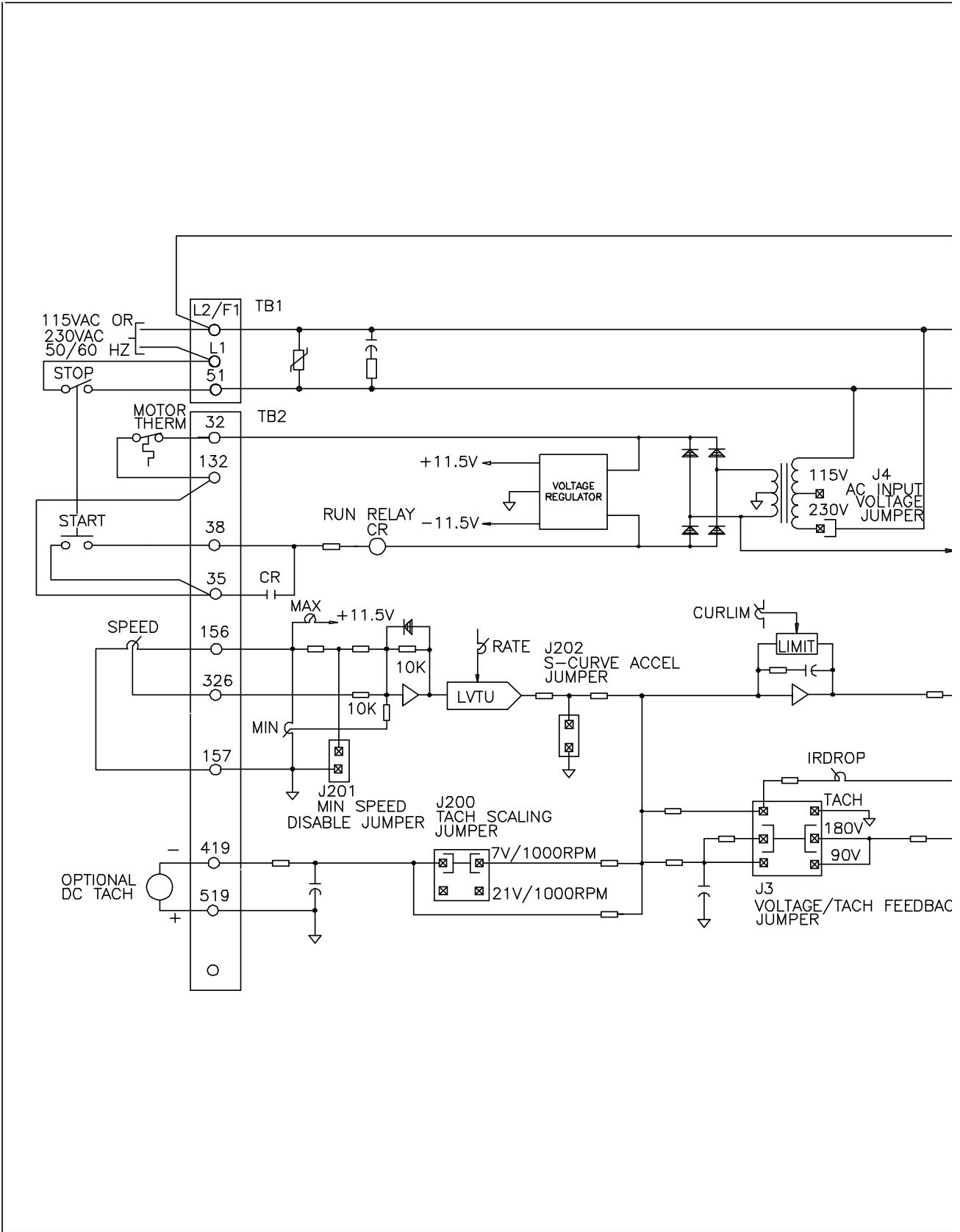
Figure 5-1. Wiring Diagram of Basic Speed Controller (0-57210-30).
