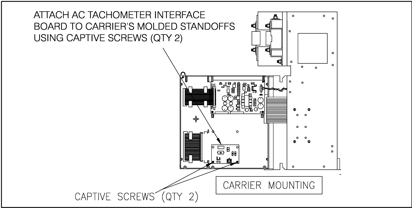
Figure 3.2 - Mounting the AC Tachometer Interface Board on the Carrier
