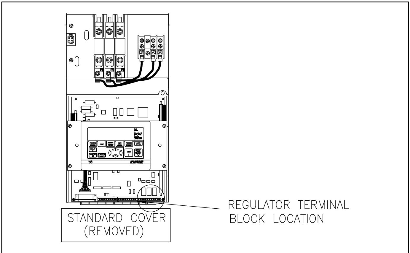
Figure 3.6 - Regulator Board Terminal Location
