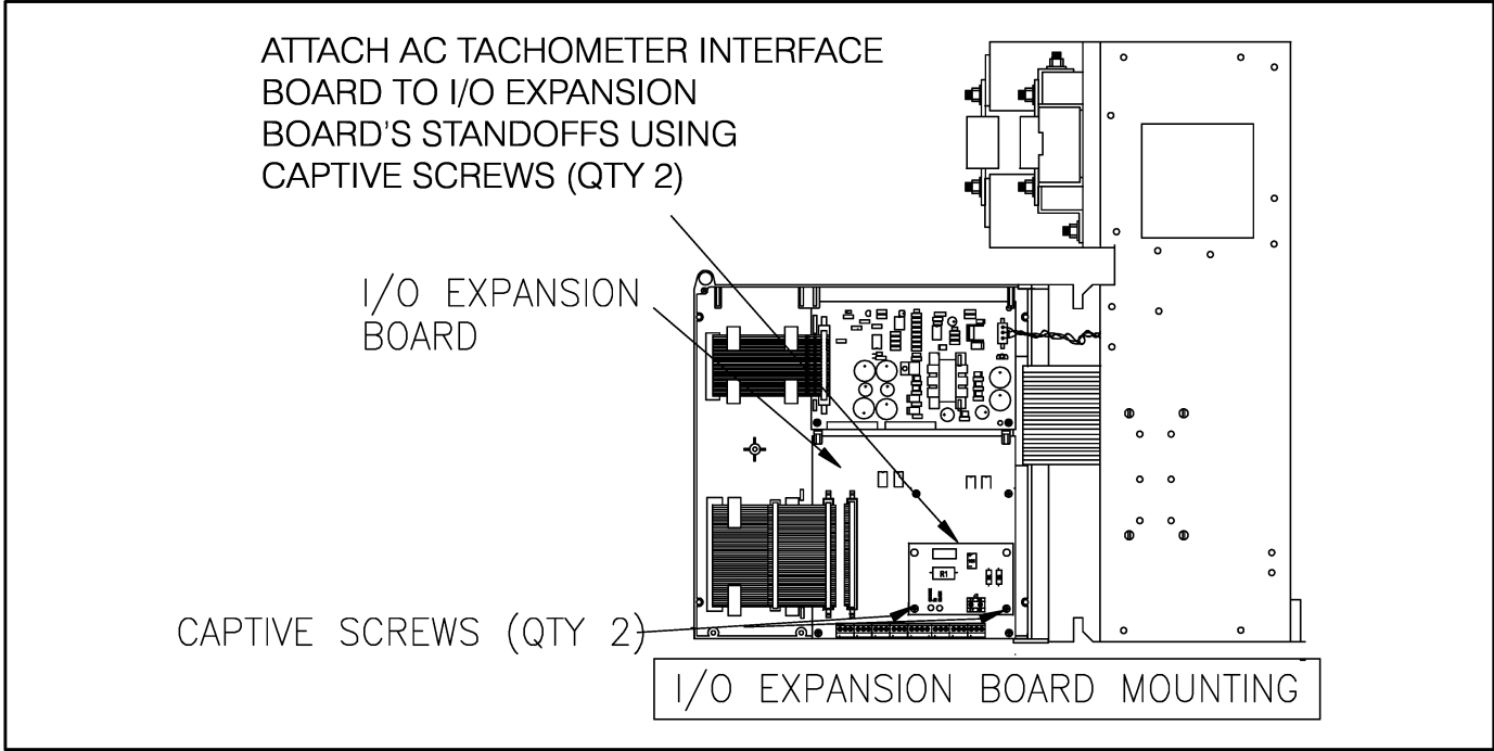
Figure 3.3 - Mounting the Interface Board on an I/O Expansion Board
