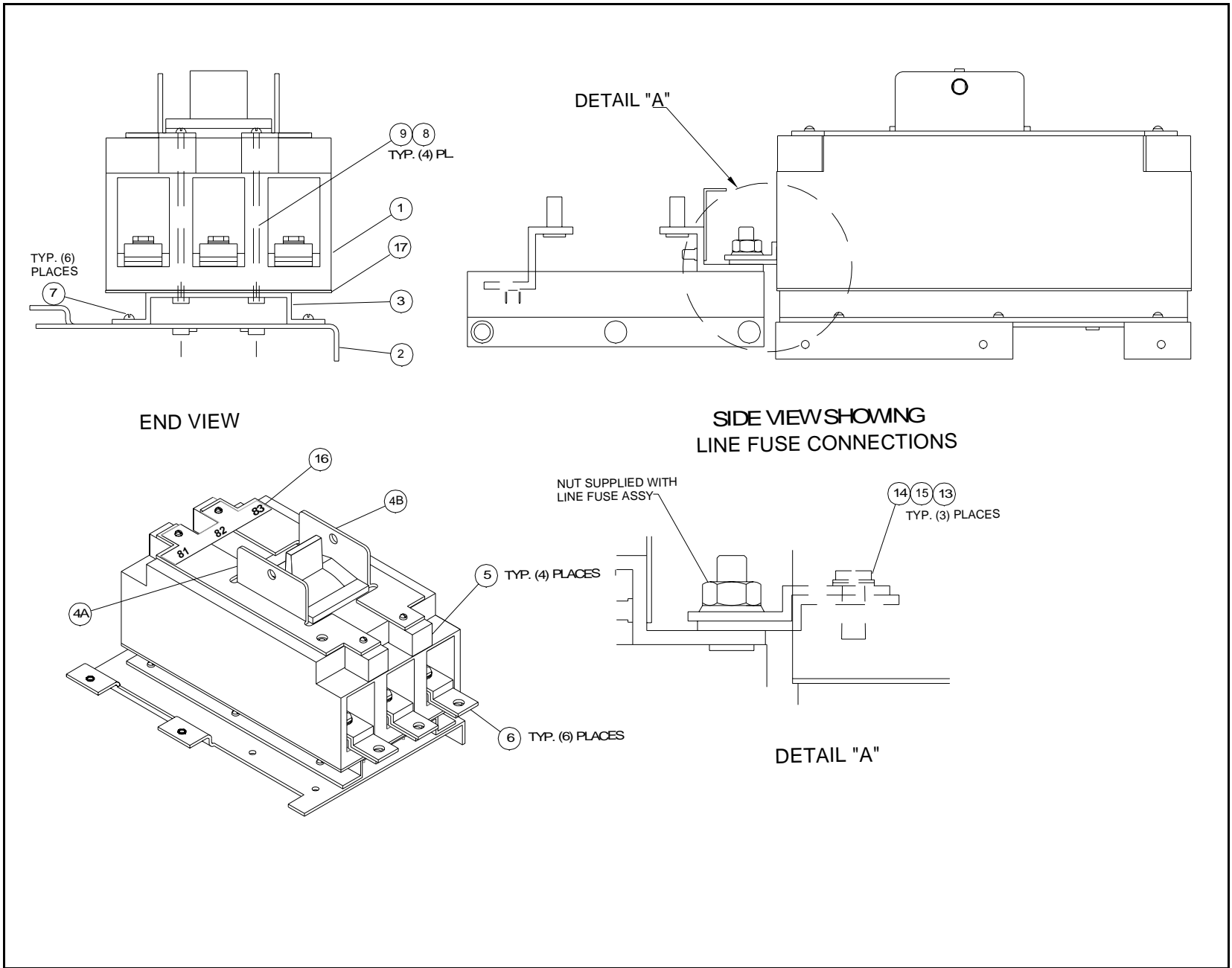
Figure 5 - 400 Amp NEMA 1 Kit (MIN 901FK1212)
