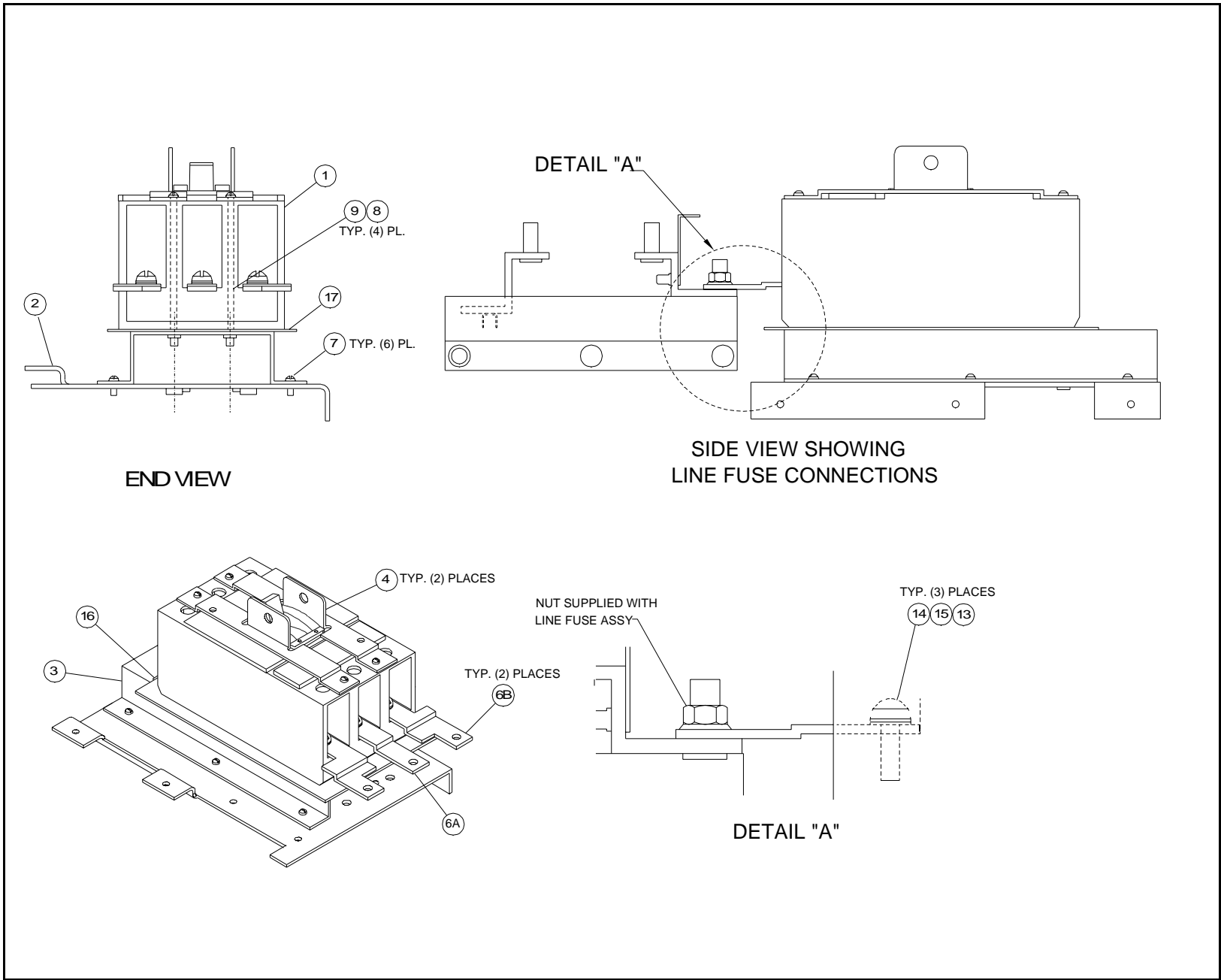
Figure 3 – 250 Amp NEMA 1 Kit (M/N 901FK1112)
